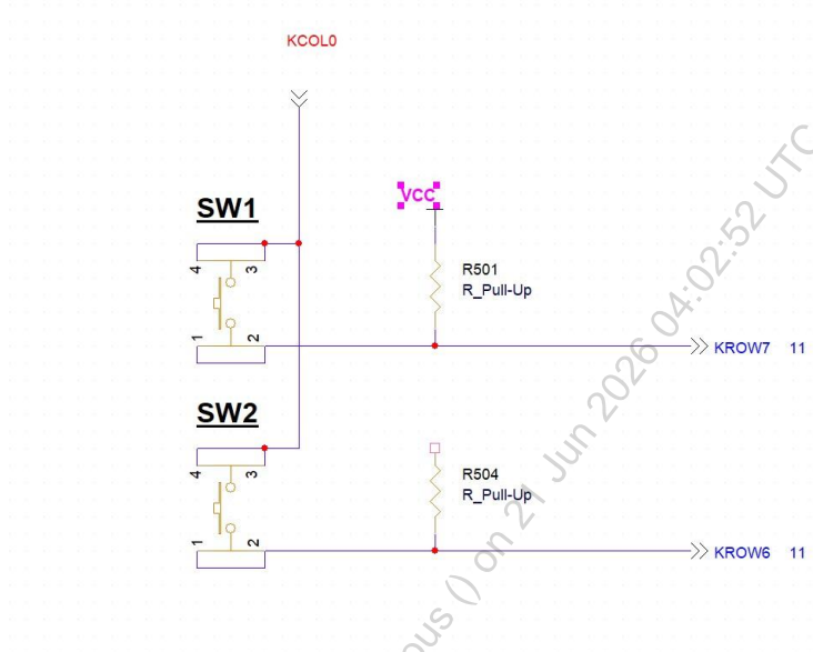
Figure 8. Input Voltage of row-input
