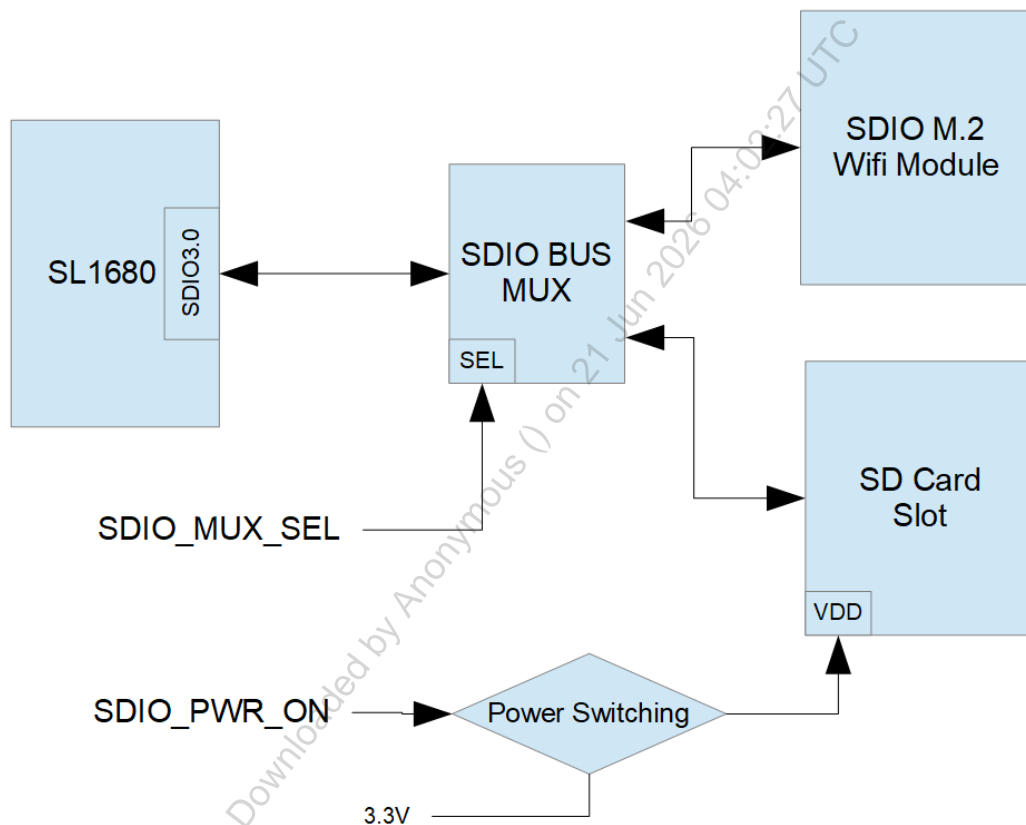
Figure 3. SDIO connection of SL1680 RDK
