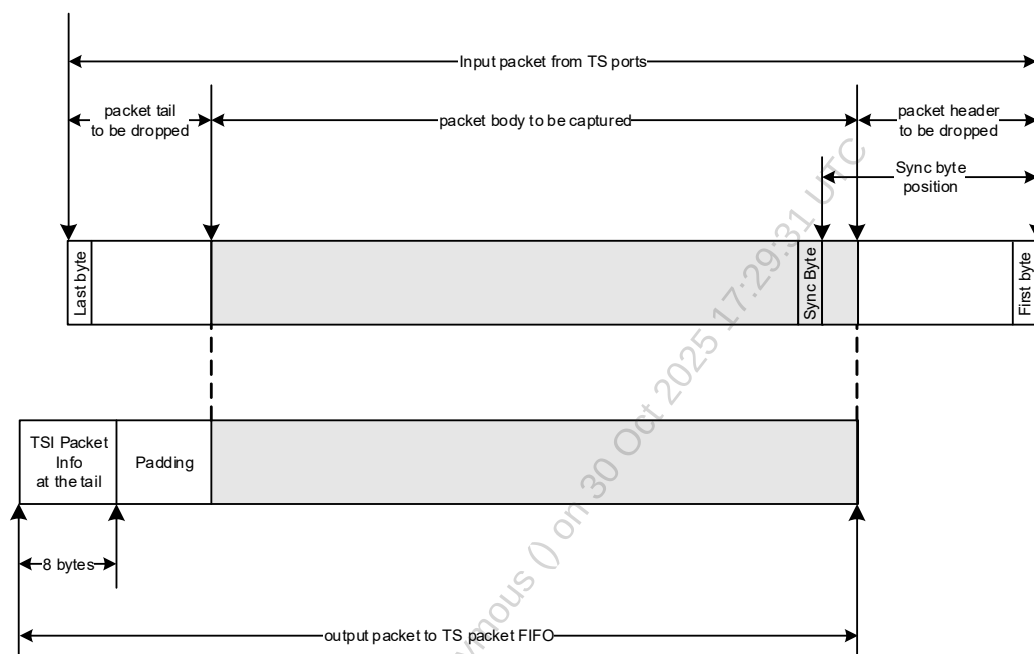
Figure 3. Input/Output packet format
