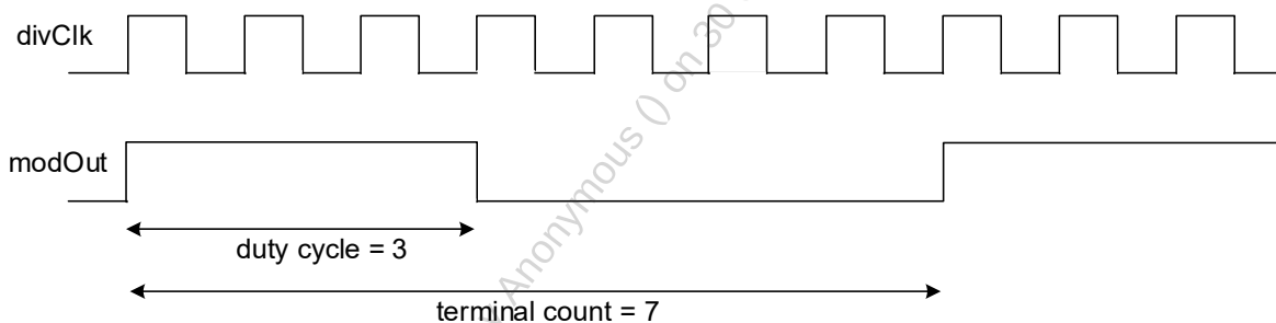
Figure 2. Waveform
