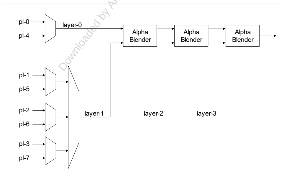
Figure 3. Block Diagram of Overlay Engine which is part of CPCB0
