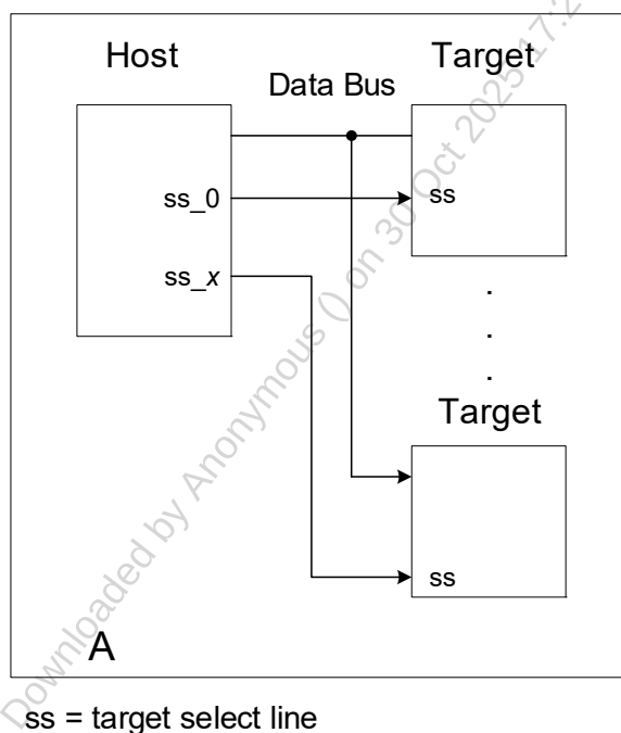
Figure 13. Hardware Target Selection
