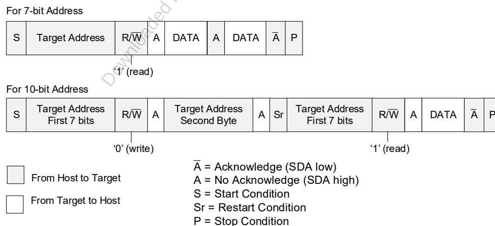
Figure 8. Host-Receiver Protocol
