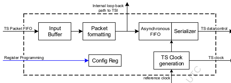
Figure 4. Transport Stream Output (TSO) Flow
