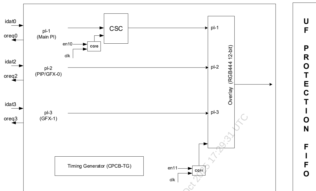
Figure 2. Detailed Block Diagram of CPCB0
